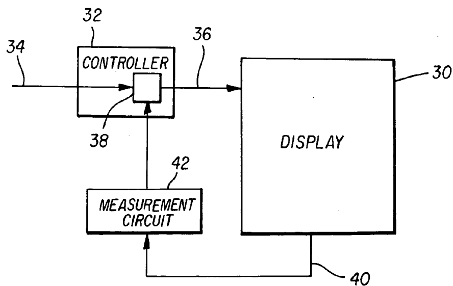
FIG. 3 (Prior Art)
